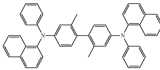
\alpha -NPB
